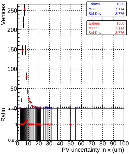
Legend: DQM_TT_ORIGINAL (black line with dots), DQM_TT_MODIFIED_propToPlane_PRVersionFINAL5 (red line with dots)
