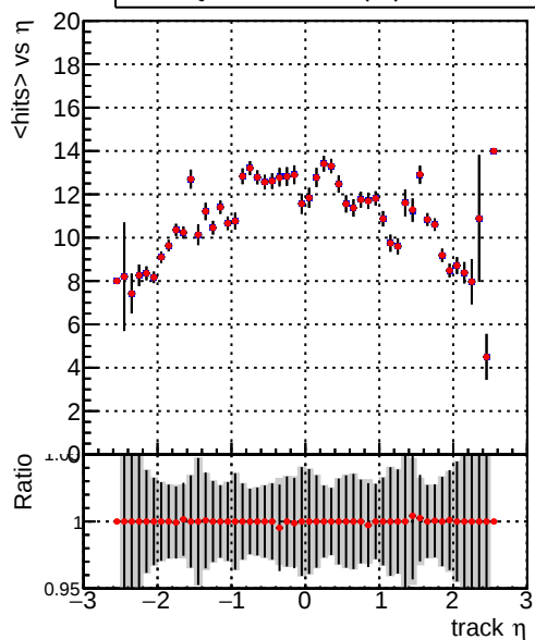
mean hits vs \eta Legend: DQM_TT_ORIGINAL (blue line with circles), DQM_TT_MODIFIED_propToPlane_PRVersionFINAL5 (red line with circles)
