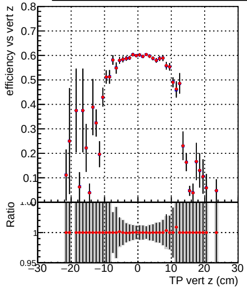
Efficiency vs TP vert z — DQM_TT_ORIGINAL — DQM_TT_MODIFIED_propToPlane_PVVersionFINAL5
