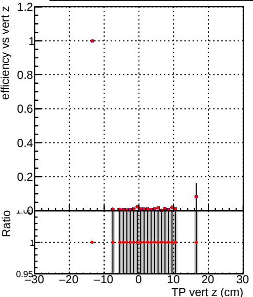
Efficiency vs vert z Legend: DQM_TT_ORIGINAL DQM_TT_MODIFIED_propToPlane_PRRVersionFINAL5
