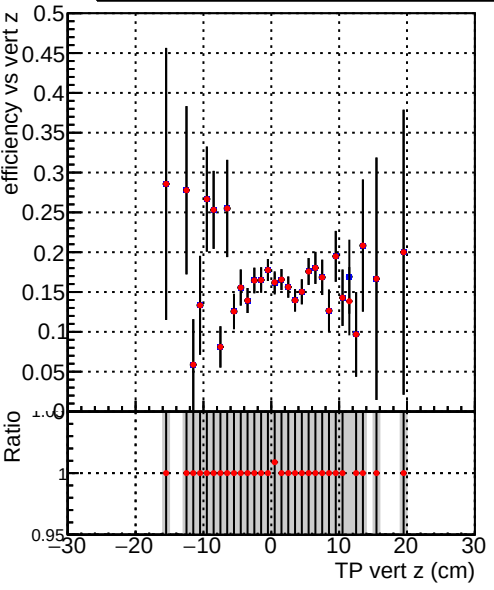
Efficiency vs TP vert z (cm) Legend: DQM_TT_ORIGINAL (blue diamond) DQM_TT_MODIFIED_propToPlane_PRRVersionFINAL5 (red diamond)
