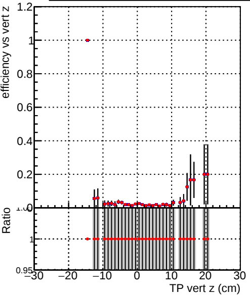
Efficiency vs TP vert z (cm) Legend: DQM_TT_ORIGINAL (grey histogram) DQM_TT_MODIFIED_propToPlane_PRRVersionFINAL5 (red line with diamonds)
