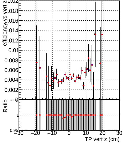
Efficiency vs. TP vert z (cm) Legend: — DQM_TT_ORIGINAL (blue line with dots) — DQM_TT_MODIFIED_propToPlane_PRVersionFINAL5 (red line with dots)
