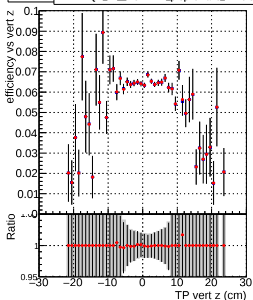
Efficiency vs TP vert z (cm) — DQM_TT_ORIGINAL — DQM_TT_MODIFIED_propToPlane_PVersionFINAL5
