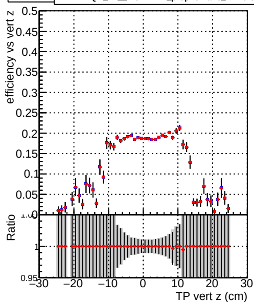
Efficiency vs. sim PV z — DQM_TT_ORIGINAL — DQM_TT_MODIFIED_propToPlane_PRRVersionFINAL5
