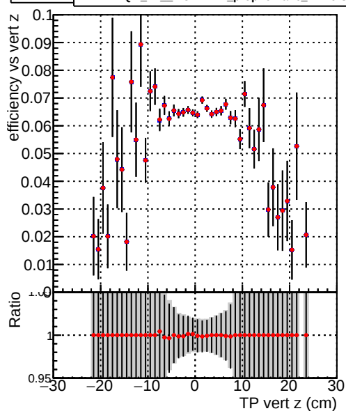
Efficiency vs. TP vert z (cm) — DQM_TT_ORIGINAL — DQM_TT_MODIFIED_propToPlane_PRRVersionFINAL5
