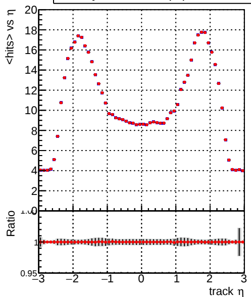
mean hit — DQM_TT_ORIGINAL — DQM_TT_MODIFIED_propToPlane_PRVersionFINAL5
