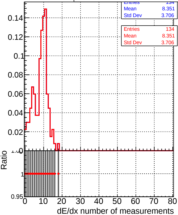
Legend for bottom row plots: DQM_TT_ORIGINAL (Blue line with squares) DQM_TT_MODIFIED_propToPlane_PRVersionFINAL5 (Red line with circles)
