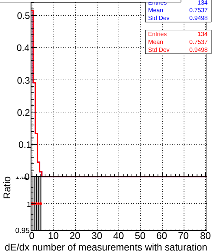
Legend for bottom row plots: DQM_TT_ORIGINAL (Blue line with squares) DQM_TT_MODIFIED_propToPlane_PRVersionFINAL5 (Red line with circles)
