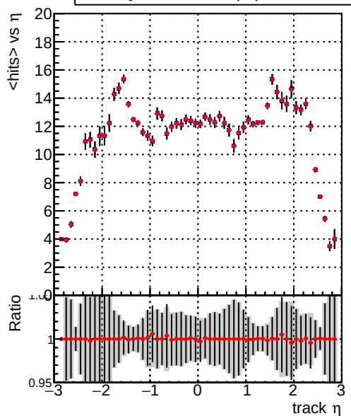
mean hits vs \eta Legend: DQM_TT_ORIGINAL (blue line with circles), DQM_TT_MODIFIED_propToPlane_PRVersionFINAL5 (red line with circles)
