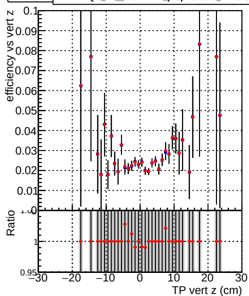
Efficiency vs. sim PV z — DQM_TT_ORIGINAL — DQM_TT_MODIFIED_propToPlane_PRVersionFINAL5
