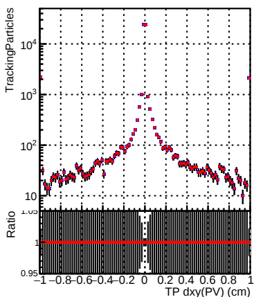
N of sim DQM_TT_ORIGINAL DQM_TT_MODIFIED_propToPlane_PVersionFINAL5
