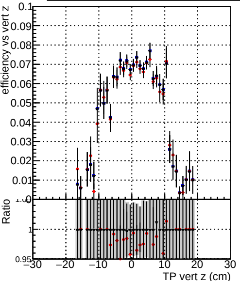
Efficiency vs TP vert z (cm) Legend: DQM_TT_ORIGINAL DQM_TT_MODIFIED_propToPlane_PVersionFINAL2 DQM_TT_MODIFIED_propToPlane_PVersionFINAL4
