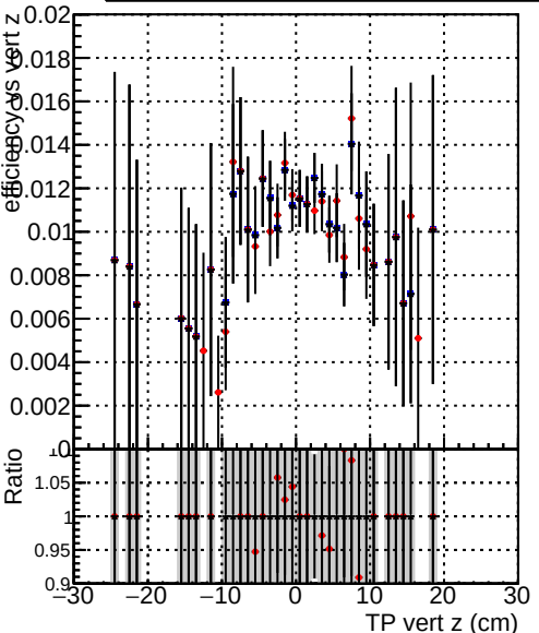
Efficiency vs TP vert z (cm) Legend: DQM_TT_ORIGINAL DQM_TT_MODIFIED_propToPlane_PRVersionFINAL2 DQM_TT_MODIFIED_propToPlane_PRVersionFINAL4
