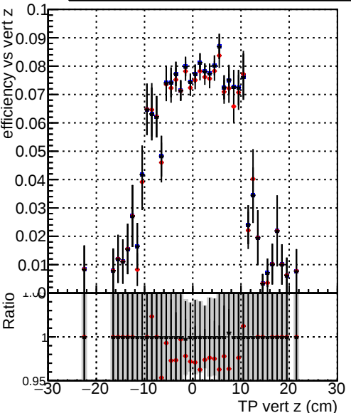
Efficiency vs vertpos Legend: DQM_TT_ORIGINAL DQM_TT_MODIFIED_propToPlane_PVersionFINAL2 DQM_TT_MODIFIED_propToPlane_PVersionFINAL4
