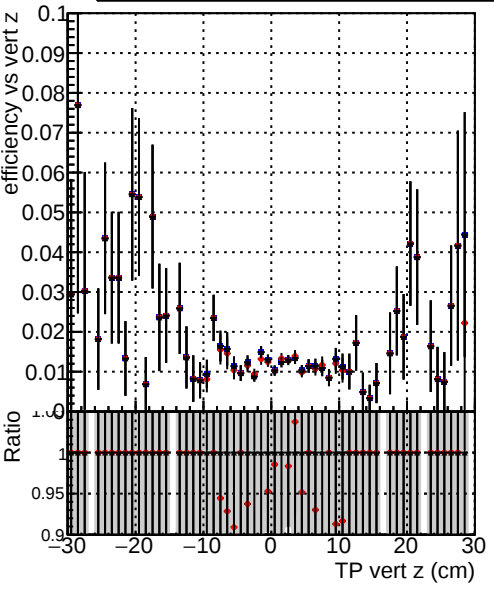
Efficiency vs vertpos Legend: DQM_TT_ORIGINAL DQM_TT_MODIFIED_propToPlane_PRRVersionFINAL2 DQM_TT_MODIFIED_propToPlane_PRRVersionFINAL4
