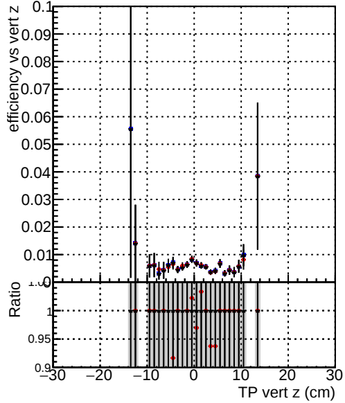
Efficiency vs. TP vert z (cm) — DQM_TT_ORIGINAL — DQM_TT_MODIFIED_propToPlane_PRRVersionFINAL2 — DQM_TT_MODIFIED_propToPlane_PRRVersionFINAL4
