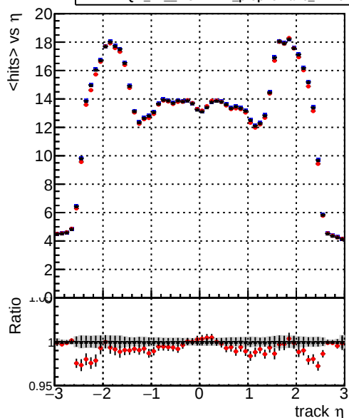
mean hits vs \eta Legend: DQM_TT_ORIGINAL (blue line), DQM_TT_MODIFIED_propToPlane_PRVersionFINAL2 (red line), DQM_TT_MODIFIED_propToPlane_PRVersionFINAL4 (black line)
