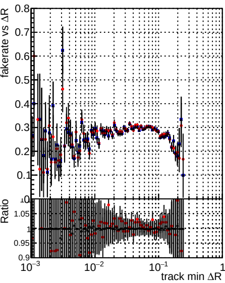
Legend: DQM TT ORIGINAL (black), DQM TT MODIFIED (red), DQM TT MODIFIED propToPlane_PRRVersionFINAL2 (blue)
