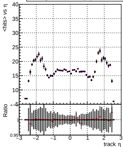
mean hits vs \eta DQM_TT_ORIGINAL DQM_TT_MODIFIED_propToPlane_PRVersionFINAL2 DQM_TT_MODIFIED_propToPlane_PRVersionFINAL4
