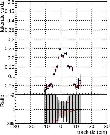
Fake rate vs dz Legend: DOM TT ORIGINAL, DOM TT MODIFIED, propToPlane, PRVersionFINAL2
