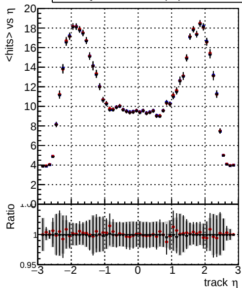
mean hit — DQM_TT_ORIGINAL — DQM_TT_MODIFIED_propToPlane_PRRVersionFINAL2 — DQM_TT_MODIFIED_propToPlane_PRRVersionFINAL4
