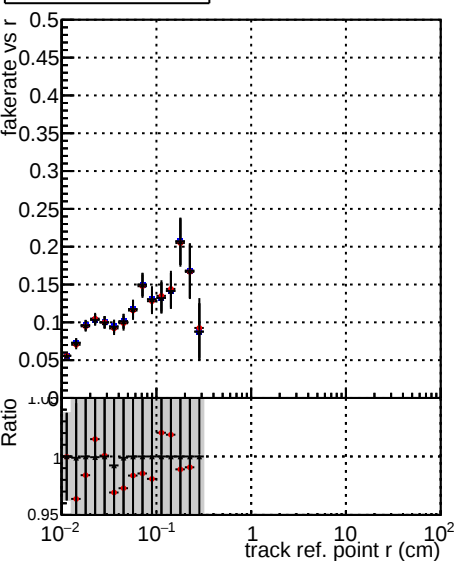
Fake rate vs verpos Legend: DOM TT ORIGINAL DOM TT MODIFIED_propToPlane_PRRVersionFINAL2 DOM TT MODIFIED_propToPlane_PRRVersionFINAL4
