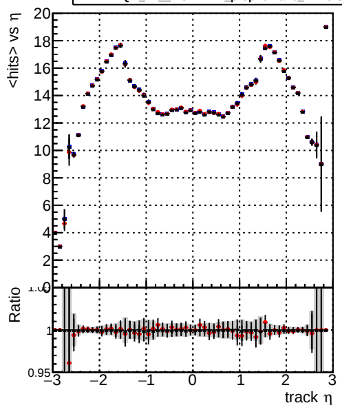
mean hits vs \eta — DQM_TT_ORIGINAL — DQM_TT_MODIFIED_propToPlane_PRVersionFINAL2 — DQM_TT_MODIFIED_propToPlane_PRVersionFINAL4
