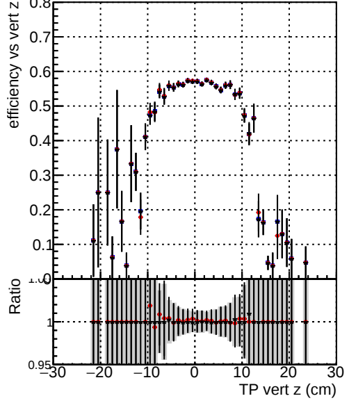
Efficiency vs. TP vert z (cm) — DQM_TT_ORIGINAL — DQM_TT_MODIFIED_propToPlane_PVersionFINAL2 — DQM_TT_MODIFIED_propToPlane_PVersionFINAL4
