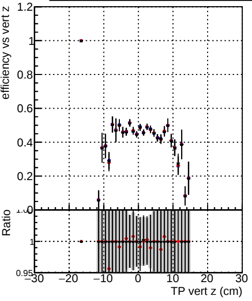
Efficiency vs vert z Legend: DQM_TT_ORIGINAL DQM_TT_MODIFIED_propToPlane_PRRVersionFINAL2 DQM_TT_MODIFIED_propToPlane_PRRVersionFINAL4
