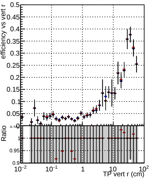
Efficiency vs TP vert r (cm) Legend: DQM_TT_ORIGINAL DQM_TT_MODIFIED_propToPlane_PRRVersionFINAL2 DQM_TT_MODIFIED_propToPlane_PRRVersionFINAL4
