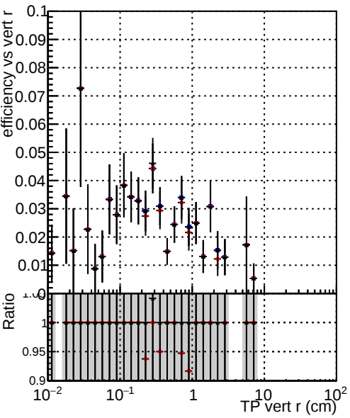
Efficiency vs TP vert r (cm) Legend: DQM_TT_ORIGINAL (Blue line with dots) DQM_TT_MODIFIED_propToPlane_PVersionFINAL2 (Red line with dots) DQM_TT_MODIFIED_propToPlane_PVersionFINAL4 (Black line with dots)
