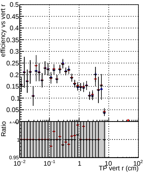
Efficiency vs vertpos Legend: DQM_TT_ORIGINAL DQM_TT_MODIFIED_propToPlane_PRVersionFINAL2 DQM_TT_MODIFIED_propToPlane_PRVersionFINAL4
