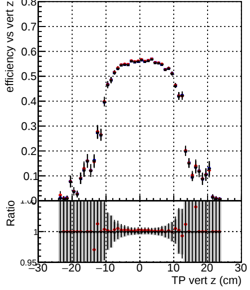
Efficiency vs. TP vert z (cm) Legend: - DQM_TT_ORIGINAL (blue dots) - DQM_TT_MODIFIED_propToPlane_PRRVersionFINAL2 (red dots) - DQM_TT_MODIFIED_propToPlane_PRRVersionFINAL4 (black dots)
