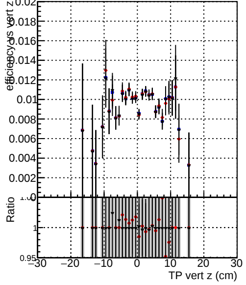
Efficiency vs. TP vert z — DQM_TT_ORIGINAL — DQM_TT_MODIFIED_propToPlane_PVersionFINAL2 — DQM_TT_MODIFIED_propToPlane_PVersionFINAL4
