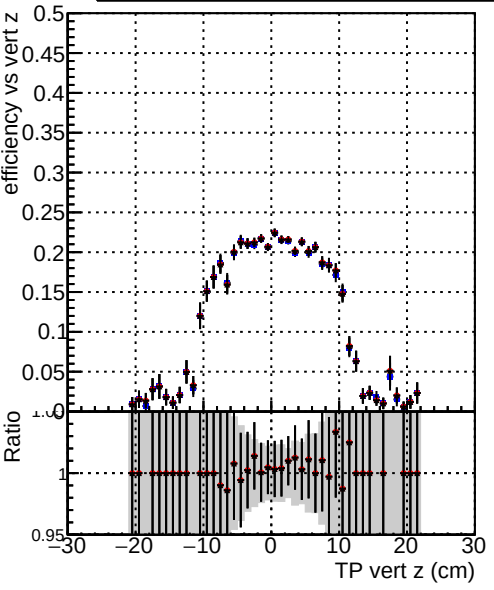
Efficiency vs vertpos Legend: DQM_TT_ORIGINAL DQM_TT_MODIFIED_propToPlane_PRRVersionFINAL2 DQM_TT_MODIFIED_propToPlane_PRRVersionFINAL3
