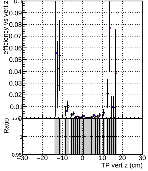
Efficiency vs vert z —●— DQM_TT_ORIGINAL —●— DQM_TT_MODIFIED_propToPlane_PRVersionFINAL2 —●— DQM_TT_MODIFIED_propToPlane_PRVersionFINAL3
