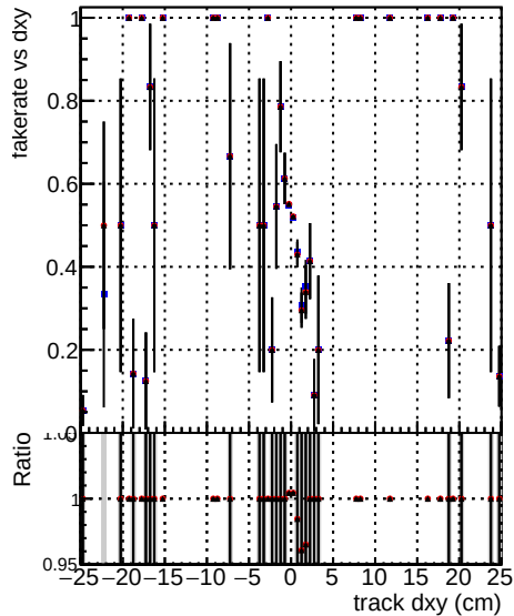
Fake rate vs d DOM TT ORIGINAL BQM TT MODIFIED propToPlane PRVersionFINAL3
