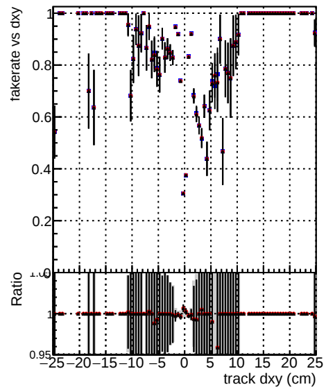
Fake rate vs d DOM TT ORIGINAL DOM TT MODIFIED propToPlane PRVersionFINAL2 propToPlane PRVersionFINAL3
