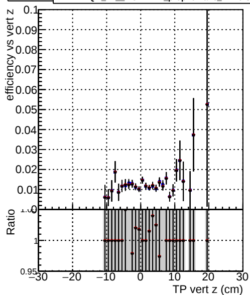
Efficiency vs. TP vert z (cm) — DQM_TT_ORIGINAL — DQM_TT_MODIFIED_propToPlane_PRRVersionFINAL2 — DQM_TT_MODIFIED_propToPlane_PRRVersionFINAL3
