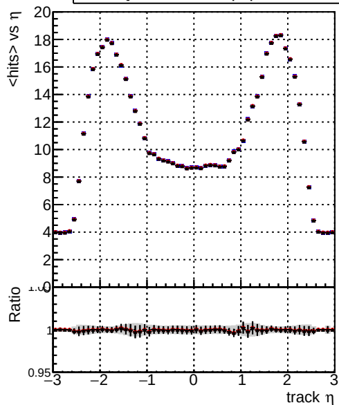
mean hit — DQM_TT_ORIGINAL — DQM_TT_MODIFIED_propToPlane_PVersionFINAL2 — DQM_TT_MODIFIED_propToPlane_PVersionFINAL3
