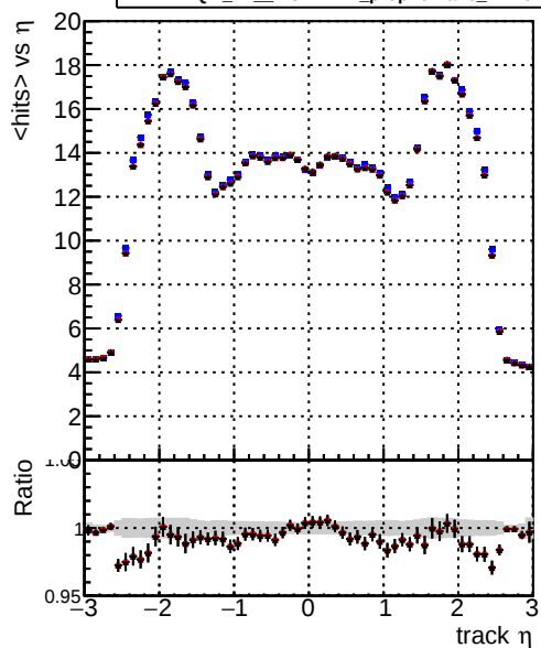
mean hits vs \eta Legend: DQM_TT_ORIGINAL (blue line), DQM_TT_MODIFIED_propToPlane_PRVersionFINAL2 (red line), DQM_TT_MODIFIED_propToPlane_PRVersionFINAL3 (black line)
