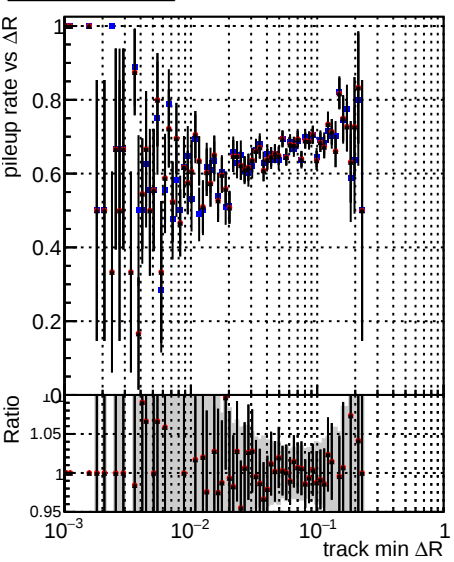
Legend: DQM TT ORIGINAL (black), DQM TT MODIFIED propToPlane_PRRVersionFINAL2 (red), DQM TT MODIFIED propToPlane_PRRVersionFINAL3 (blue)
