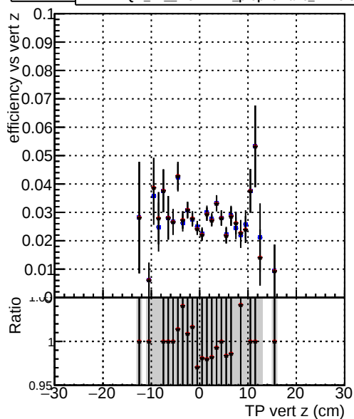
Efficiency vs. sim PV z —•— DQM_TT_ORIGINAL —•— DQM_TT_MODIFIED_propToPlane_PVersionFINAL2 —•— DQM_TT_MODIFIED_propToPlane_PVersionFINAL3
