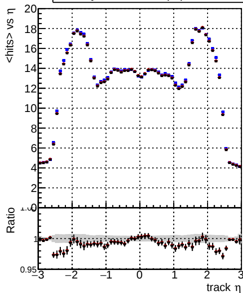
mean hits vs \eta — DQM_TT_ORIGINAL — DQM_TT_MODIFIED_propToPlane_PRVersionFINAL2 — DQM_TT_MODIFIED_propToPlane_PRVersionFINAL3
