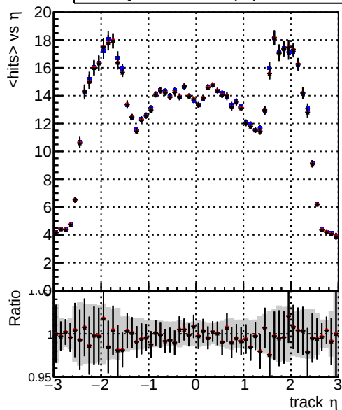
mean hits — DQM_TT_ORIGINAL — DQM_TT_MODIFIED_propToPlane_PVersionFINAL2 — DQM_TT_MODIFIED_propToPlane_PVersionFINAL3
