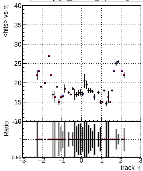
mean hit — DQM_TT_ORIGINAL — DQM_TT_MODIFIED_propToPlane_PRRVersionFINAL2 — DQM_TT_MODIFIED_propToPlane_PRRVersionFINAL3
