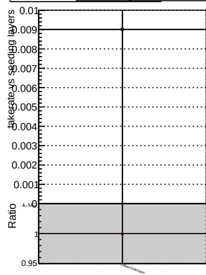
Fake rate vs. DOM TT ORIGINAL propToPlane PRVersionFINAL2 DOM TT MODIFIED propToPlane PRVersionFINAL3
