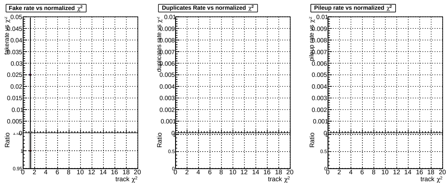
Fake rate vs. DOM TT ORIGINAL propToPlane PRVersionFINAL2 DOM TT MODIFIED propToPlane PRVersionFINAL3
