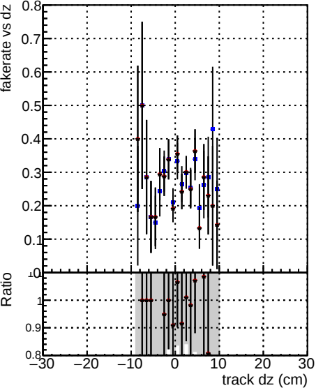
Fake rate vs dz Legend: DOM TT ORIGINAL (blue dots), DOM TT MODIFIED (red dots), propToPlane PRVersionFINAL2 (black line)
