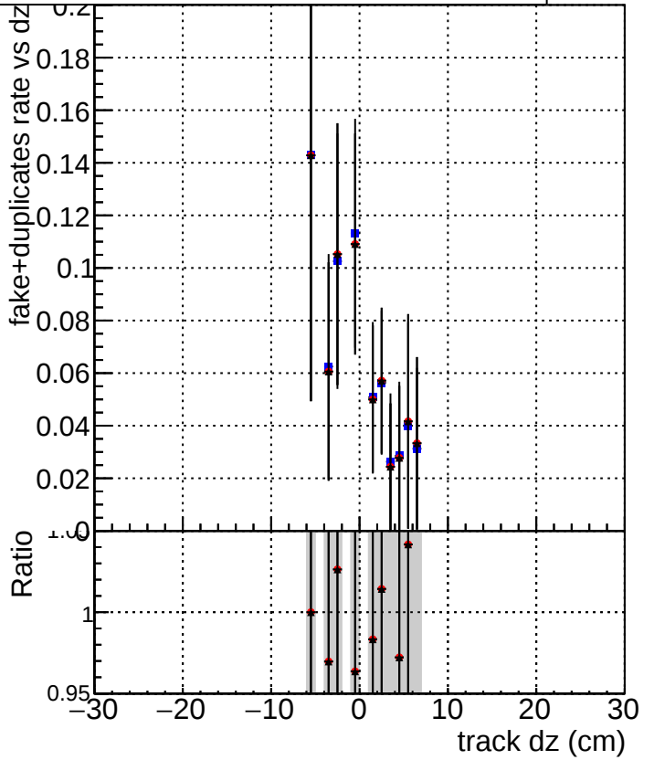
Legend for the bottom plot: DQM_TT_ORIGINAL (Blue square) DQM_TT_MODIFIED_propToPlane_PRVersionFINAL2 (Red circle) DQM_TT_MODIFIED_propToPlane_PRVersionFINAL3 (Black triangle)
