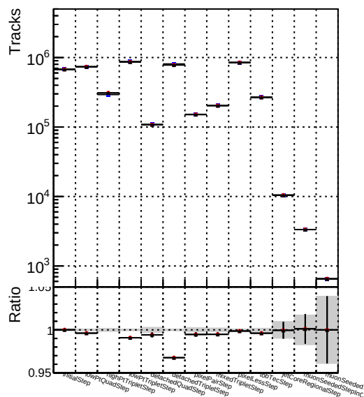
Number of tracks vs collection Legend: DQM_TT_ORIGINAL DQM_TT_MODIFIED_propToPlane_PRVersionFINAL2 DQM_TT_MODIFIED_propToPlane_PRVersionFINAL3
